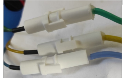
Motor power cables. There are very thin cables going to the motor
